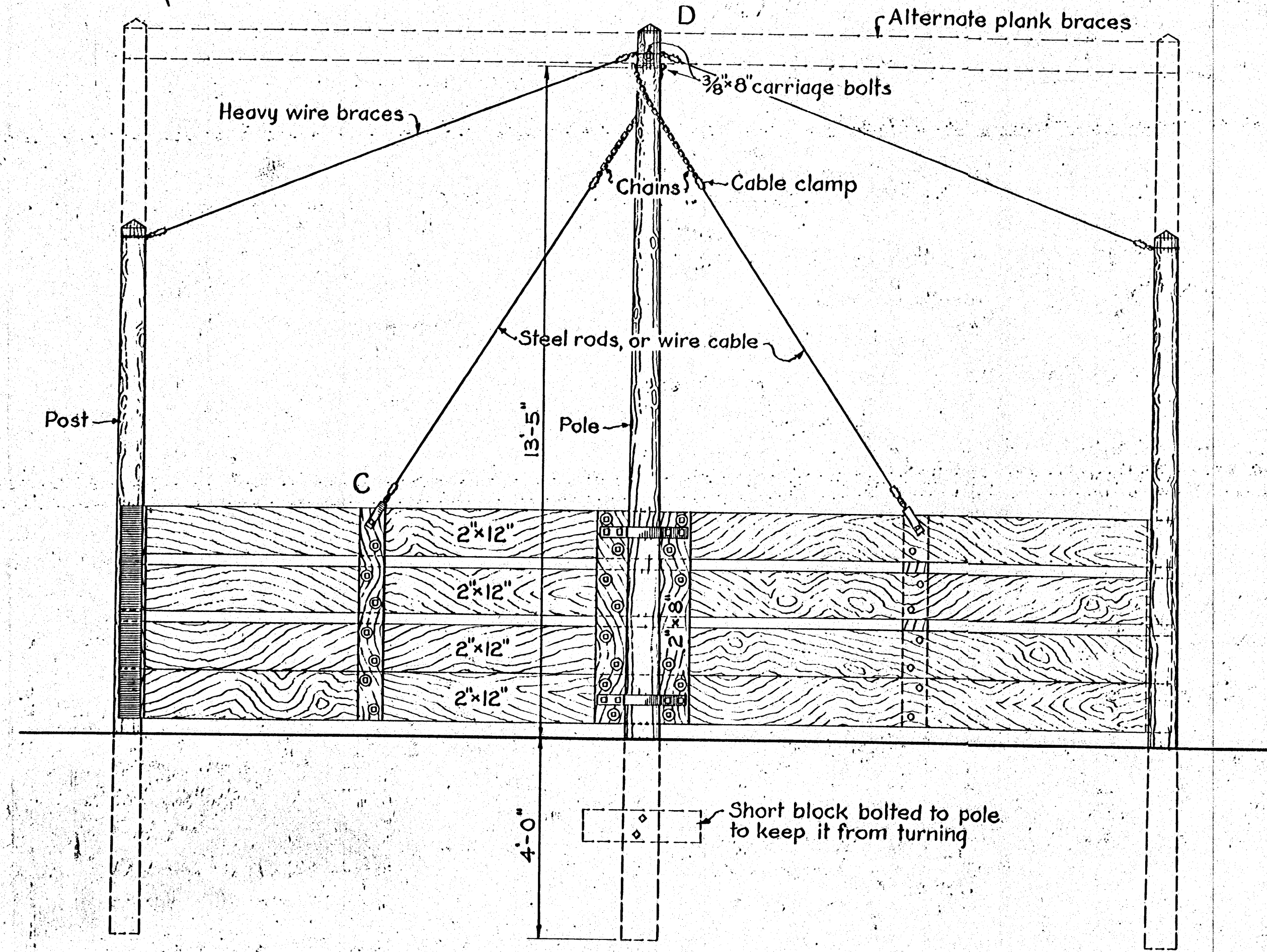
ELEVATION Scale 1/2" = 1'-0"
