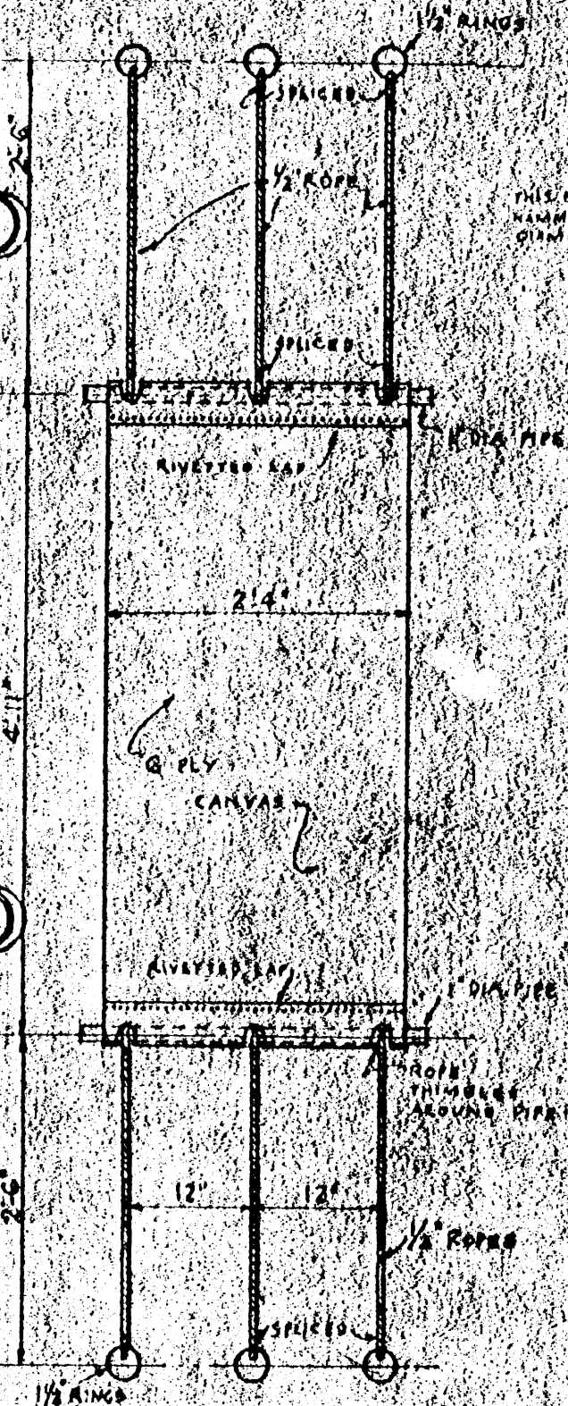
CANVAS SLING
