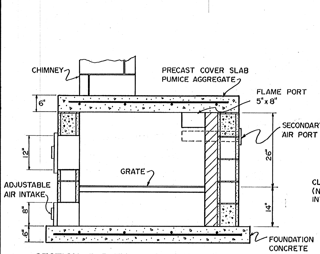
SECTION B-B THRU IGNITION CHAMBER
