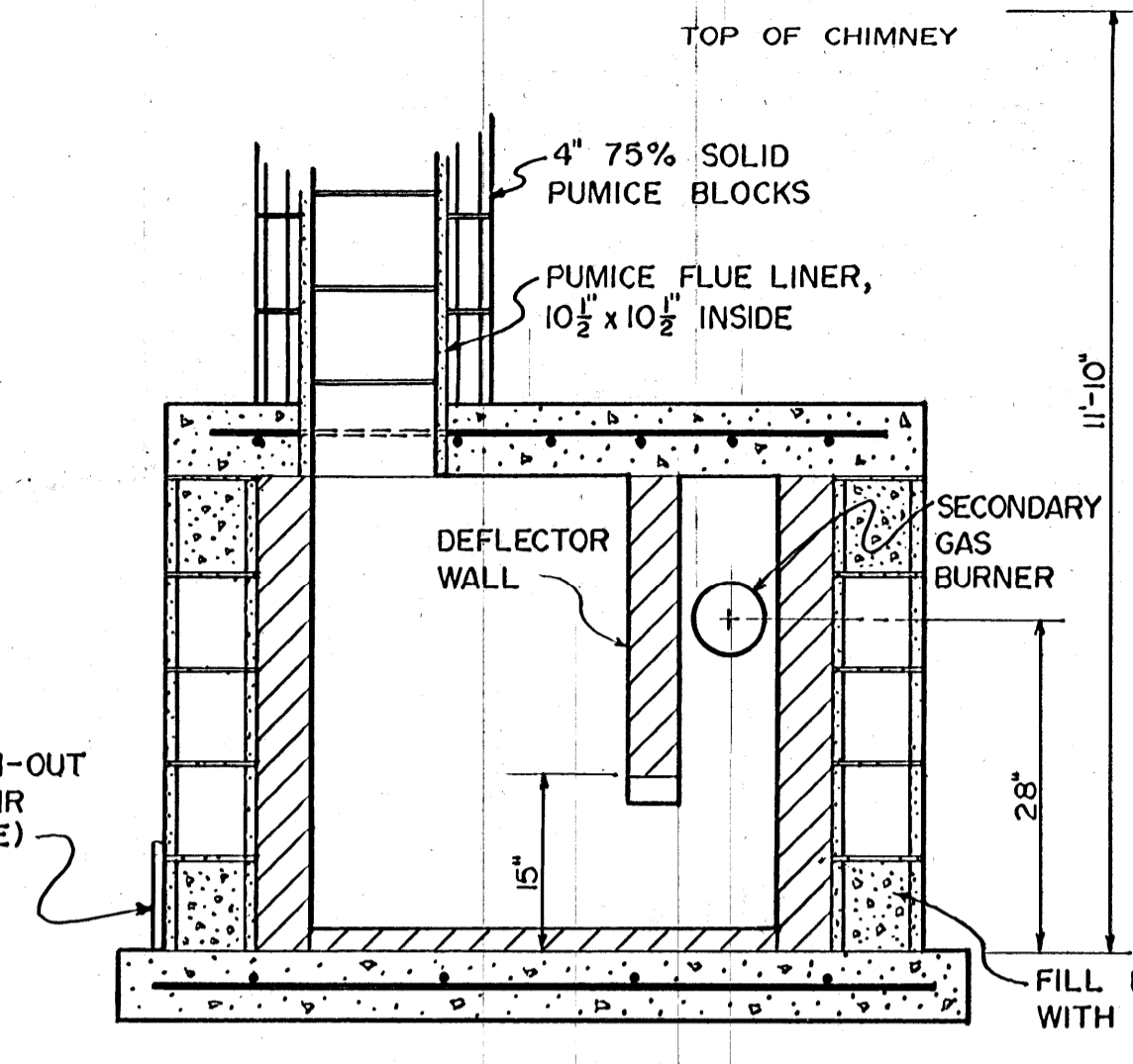
SECTION A-A THRU MIXING & COMBUSTION CHAMBERS
