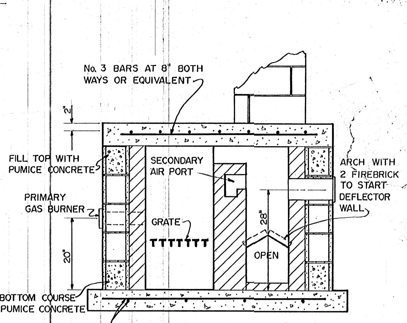
SECTION C-C THRU IGNITION & MIXING CHAMBERS
