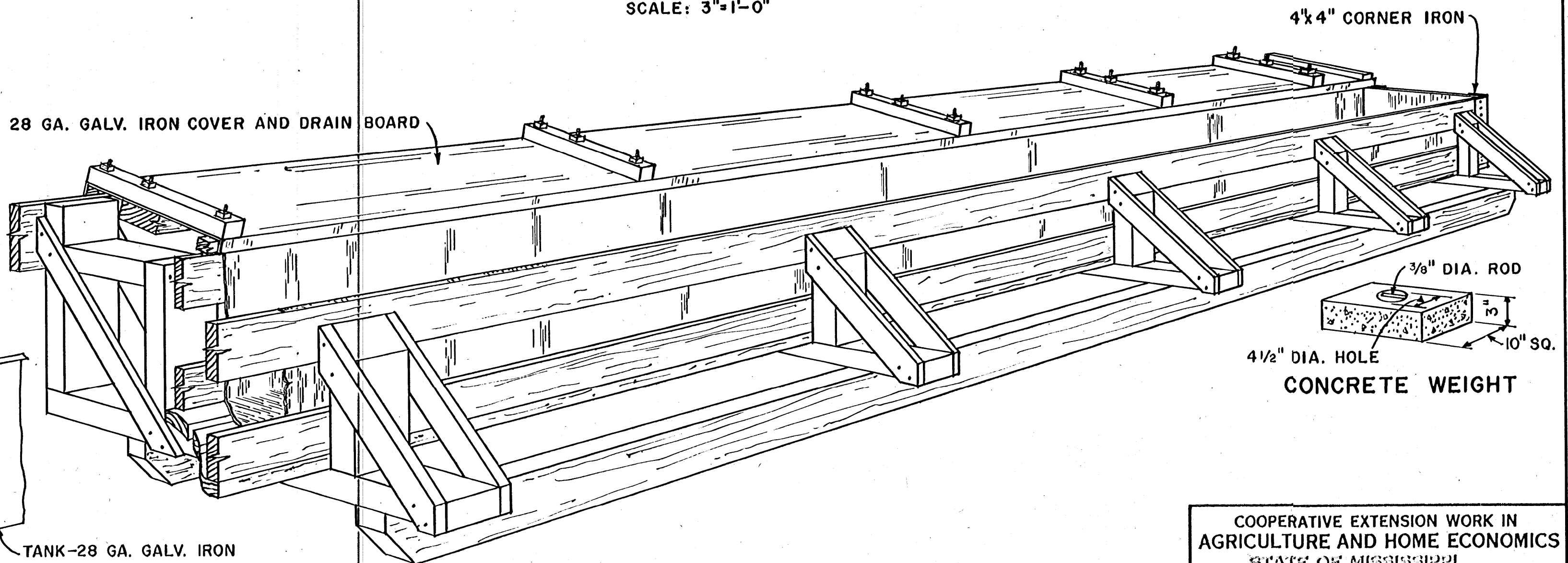
CUTAWAY PERSPECTIVE
