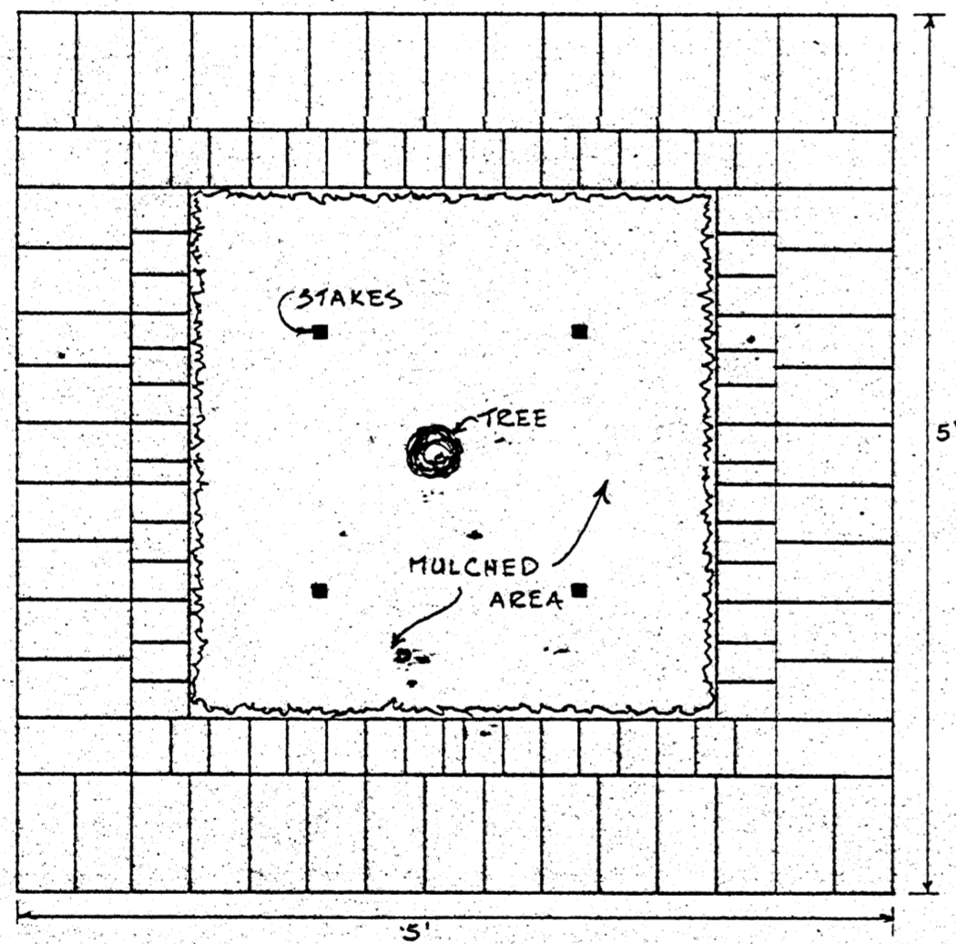
TREE PLANTING DETAIL FOR LARGE TREES
