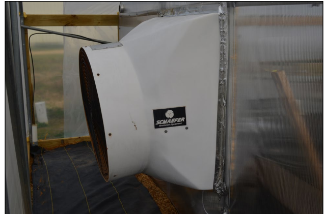
Figure 10. A 36-inch exhaust fan pulls air through a greenhouse from intake vents for temperature control.
